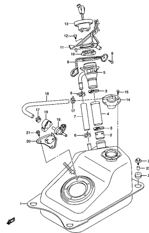
UL250K9 000_035 FUEL TANK
