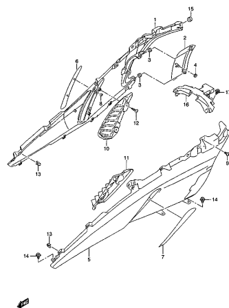
UL250K9 000_037 SIDE FRAME COVER
